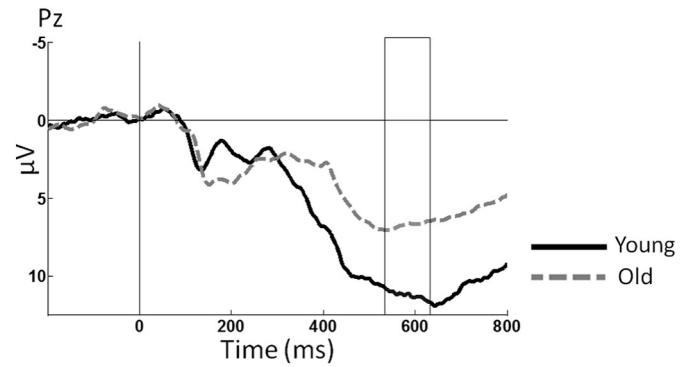
Fig. 2. Grand-average ERP waveforms at midline electrode site Pz in response to target stimuli. The rectangle indicates the approximate temporal interval in which the average amplitude was measured for the P3b.
